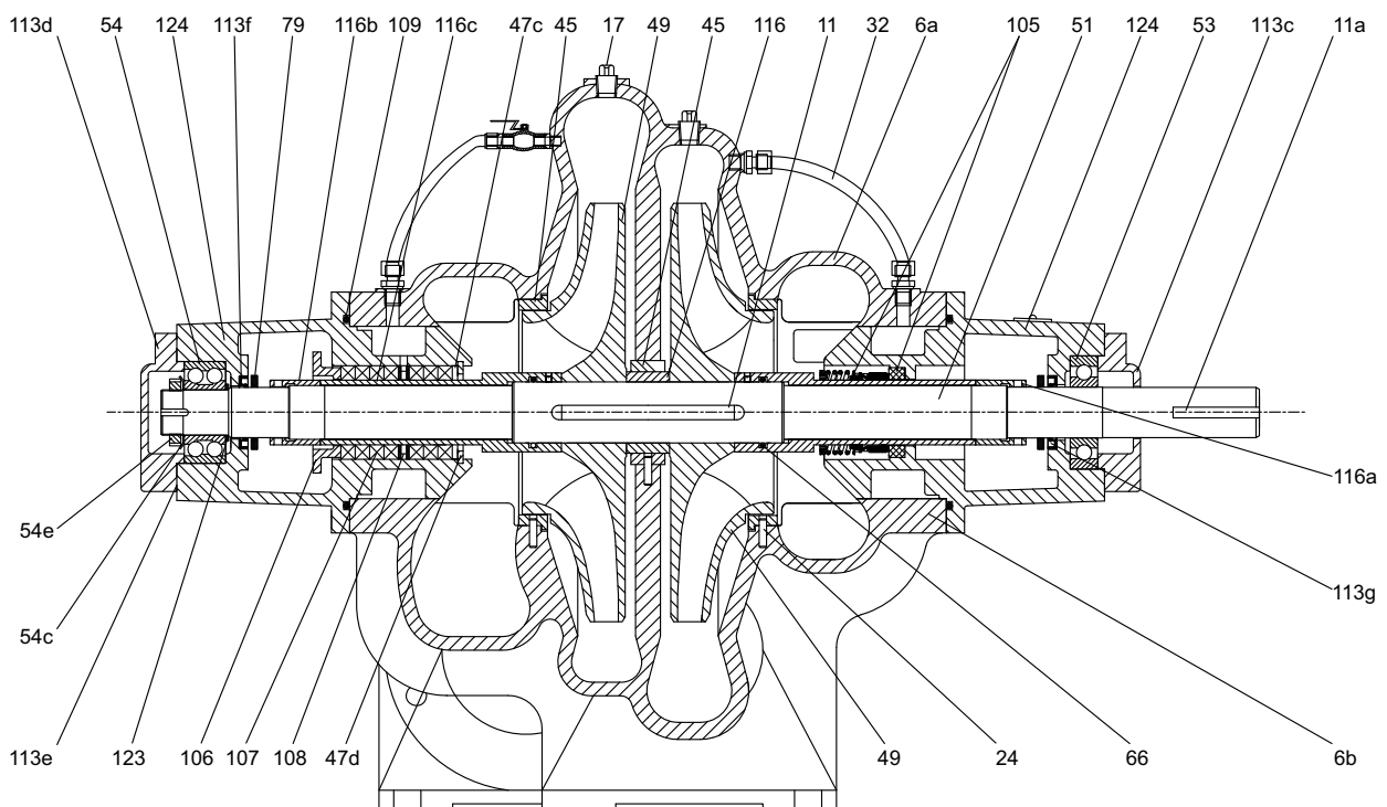
Fig. 10 Sectional drawing, standard construction type 3
