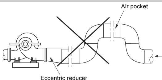
Fig. 33 Inlet pipe resulting in air pockets
