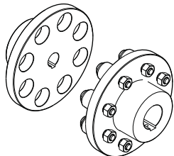
Fig. 19 Flexible pin and bush coupling
