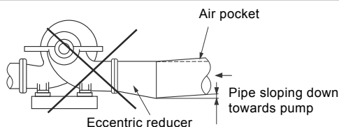
Fig. 31 Inlet pipe resulting in air pockets
