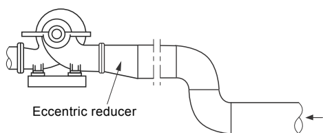
Fig. 32 Correctly mounted inlet pipe
